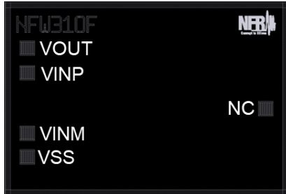
Figure 8 – Scale diagram of NFW310F. Overall dimensions are 850 \mu\text{m} by 580 \mu\text{m}
