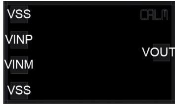
Figure 8 – Scale diagram of NFW310M. Overall dimensions are 850 \mu\text{m} by 500 \mu\text{m}
