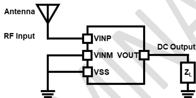
Figure 2 – Application Schematic
